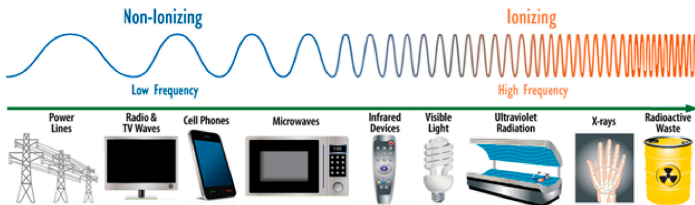
Fig. 1. Electromagnetic Spectrum (source: https://deq.utah.gov/waste-management-and-radiation-control/non-ionizing-radiation = date accessed 10th March 2023).
